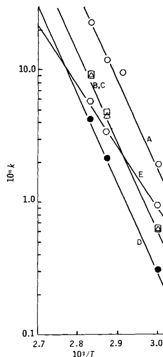
Figure 5—Arrhenius plots for A, ribose; B, xylose; C, lyxose; D, arabinose; and E, furfural in 1.00 M HCl. k is in absorbance units \cdot l. ^2 /mole ^2 \cdotsec. and n = 6 for A-D, n = 7 , and k is in absorbance units/sec. for E.
